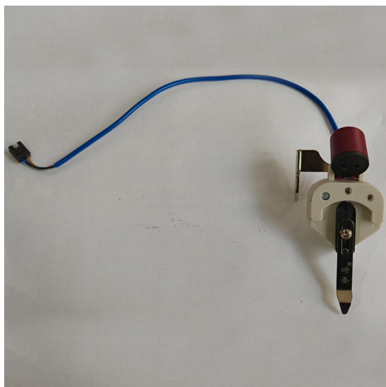
Electronic infrared probe/ Type : QS
